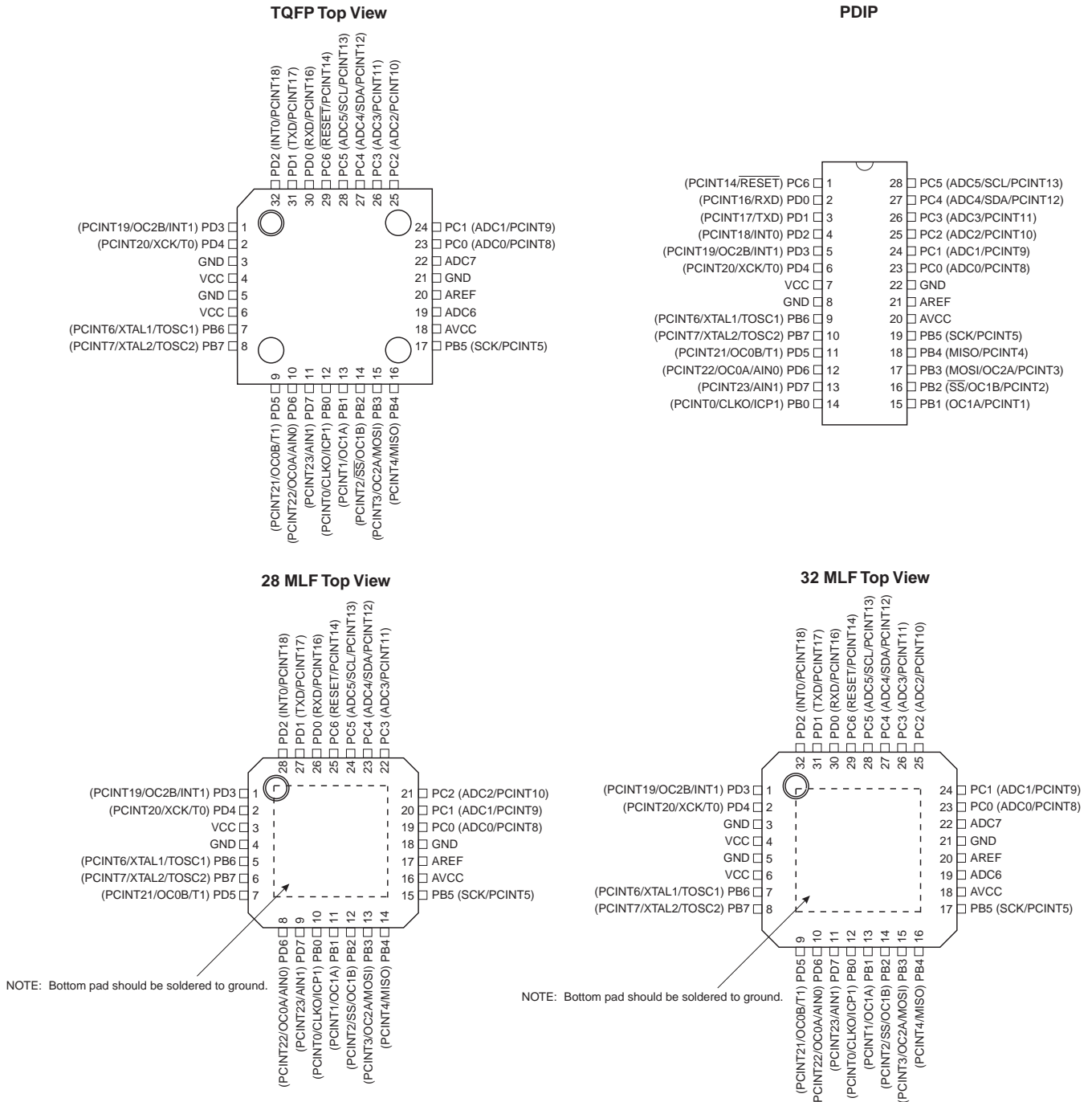
Figure 1-1. Pinout ATmega48/88/1682545PS
